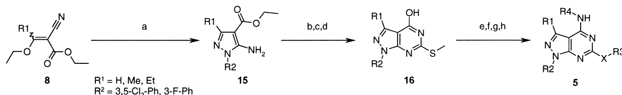
Scheme 3. (a) R 2 NHNH 2 ·HCl 14 , NEt 3 , MeOH, refl., 3 h, 58–97%; (b) PhCOCl, KSCN, acetone, refl., 3–12h, 78–100%; (c) NaOH, MeOH, refl., 2 h, 54–100%; (d) MeI, NaOH, MeOH, H 2 O, rt, 2–12h, 63–100%; (e) POCl 3 , NEt 2 iPr, refl., 1 h, 78–99%; (f) NH 3 gas or NH 2 R 4 , DMF or THF, rt, 12h, 59–99%; (g) MCPBA, THF, 0 °C to rt, 12 h, 64–92%; (h) NaH, HXR 3 , DMF, 70 °C, 11–97%.
